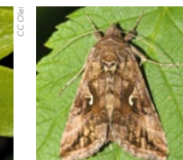
Gamma
